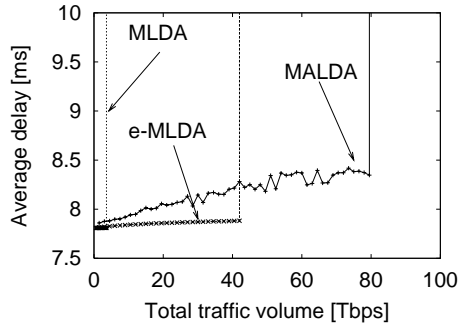
Figure 6 The average delay with traffic pattern P_1 : \mu = 16 Tbps
