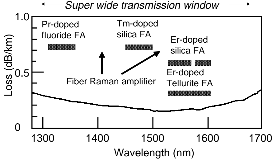
Figure 1 Loss Spectrum of Typical Low-Loss Optical Fiber
