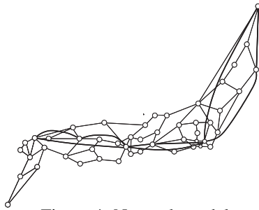
Figure 4: Network model
