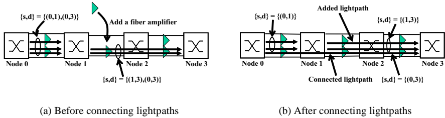
Figure 3: An example of connecting lightpaths
