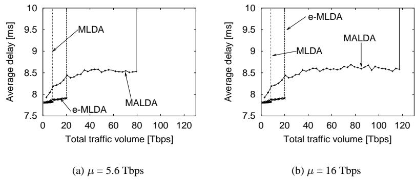
Figure 6: Average delay with traffic pattern P_2
