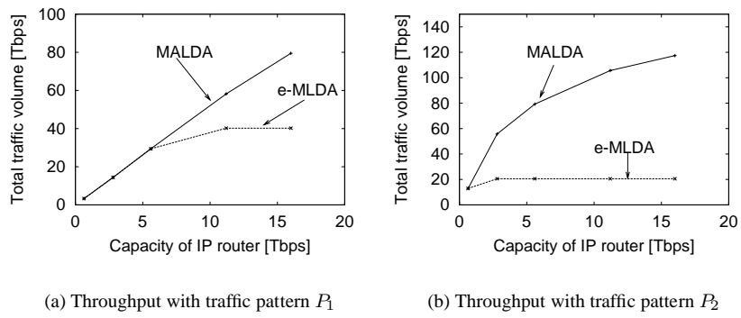
Figure 7: Throughput of each logical topology
