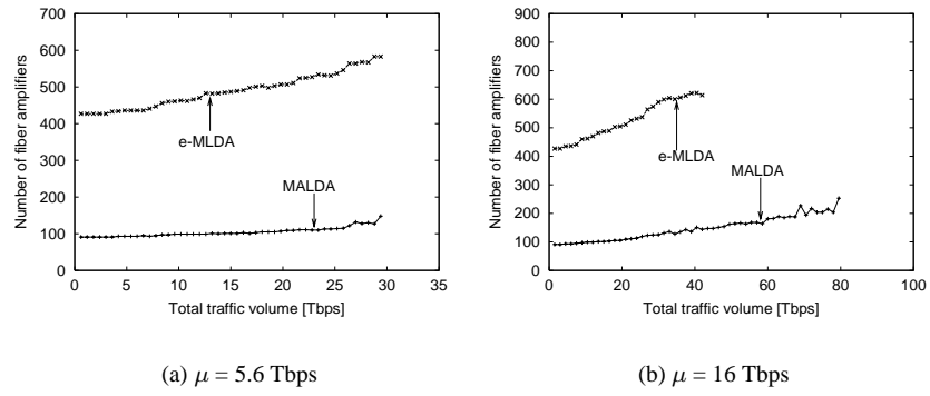
Figure 8: Number of optical fiber amplifiers needed by each logical topology with traffic pattern P_1
