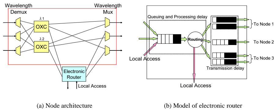
Figure 2: Node architecture model
