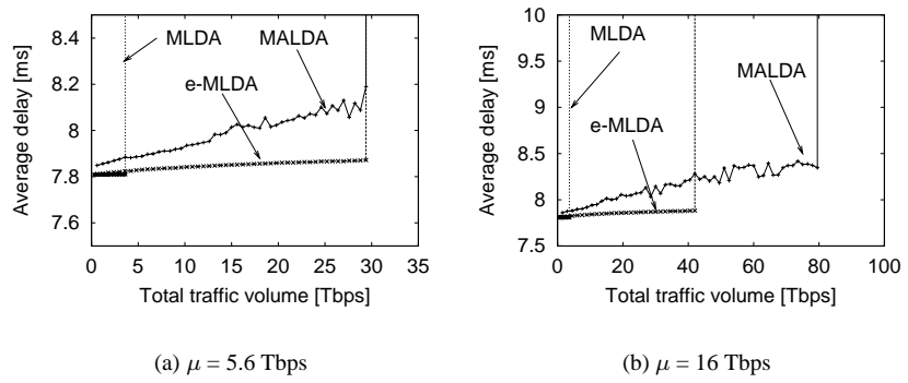
Figure 5: Average delay with traffic pattern P_1
