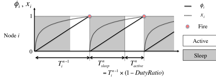
Fig. 3. Duty cycling
